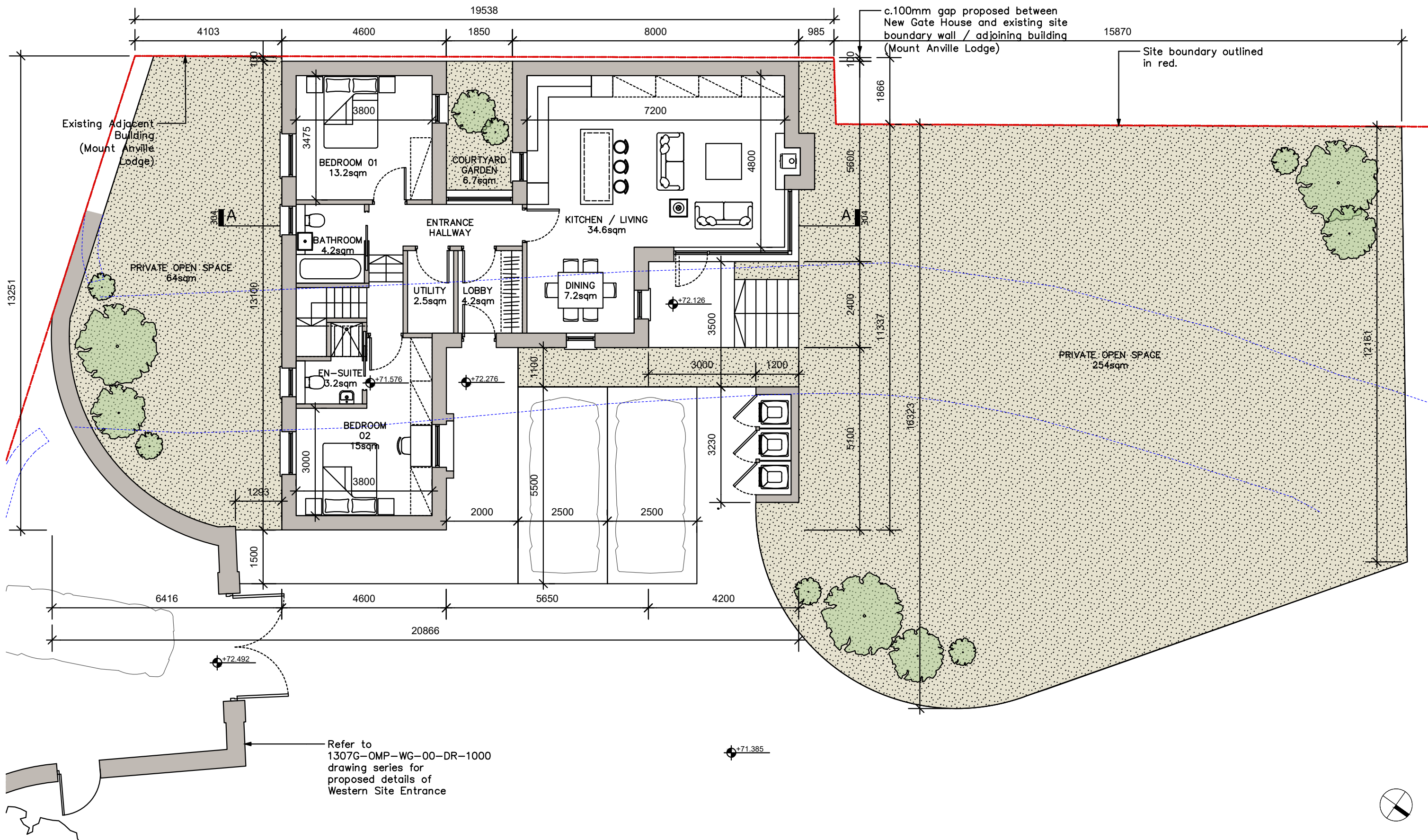
Gate House, Proposed Ground Floor Plans
